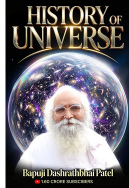
History of Universe
